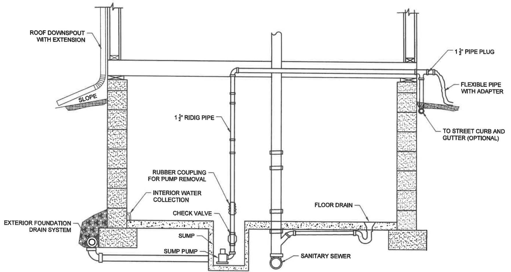
TYPICAL SUMP PUMP INSTALLATION DETAILS
